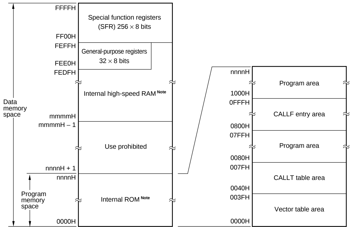
Figure 4-1. Memory Map
